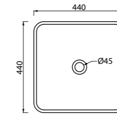
_LAVABO MONOBLOCCO QUBE 7 IN SOLID SURFACE
