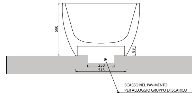
_VASCA QUADRA IN SOLID SURFACE
