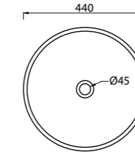
_LAVABO MONOBLOCCO FLAT 6 IN SOLID SURFACE
